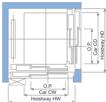
Floor plan With two entrances at 90°
